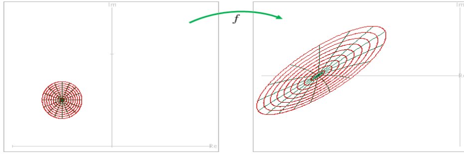
FIGURE 1. The image of |z + \frac{1-i}{2}| < \frac{1}{5} under f = z + \frac{1}{2}z^2 - \frac{i}{2}z - \frac{i}{4}z^2 \in \mathcal{UFS}_H^* .
